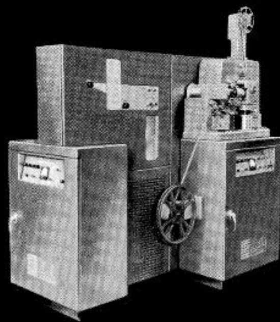
The G-E "flying spot" scanner channel Type PE-12-C handles film and slides in monochrome and color with equal operating ease. No registration or variable density problems—low operating and maintenance costs. New AGC system makes it unnecessary for the operator to ride gain under most conditions. Automatic shrinkage compensator, automatic focusing produce an undistorted, clear picture at all times.
