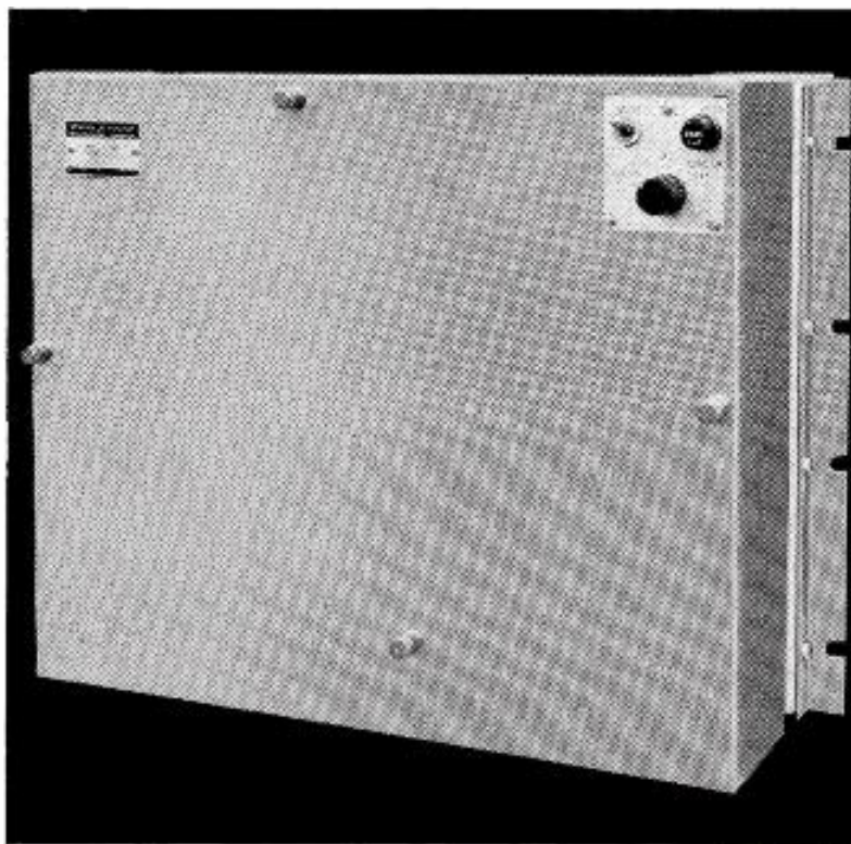
G.E.'s new transistorized sync generator the Type PG-4-B, features low power consumption, high stability and low heat output. Takes only 14 inches of rack space; built-in power supply operates from a 90 to 135 volt input.
